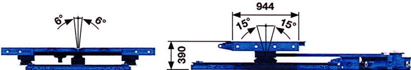
100 T/200 T TURNTABLE
