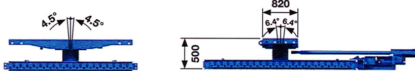
300 T/400 T TURNTABLE
